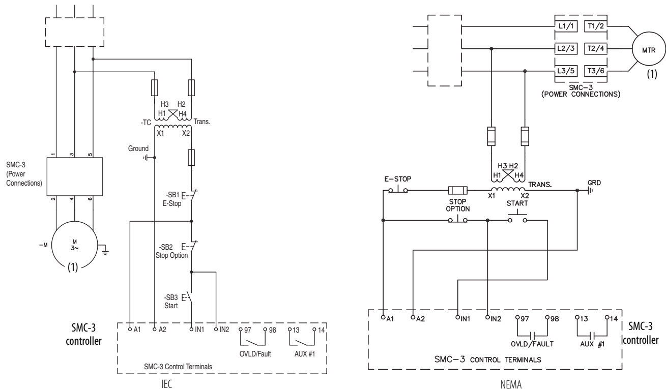
Figure 2 - Three-wire Configuration
