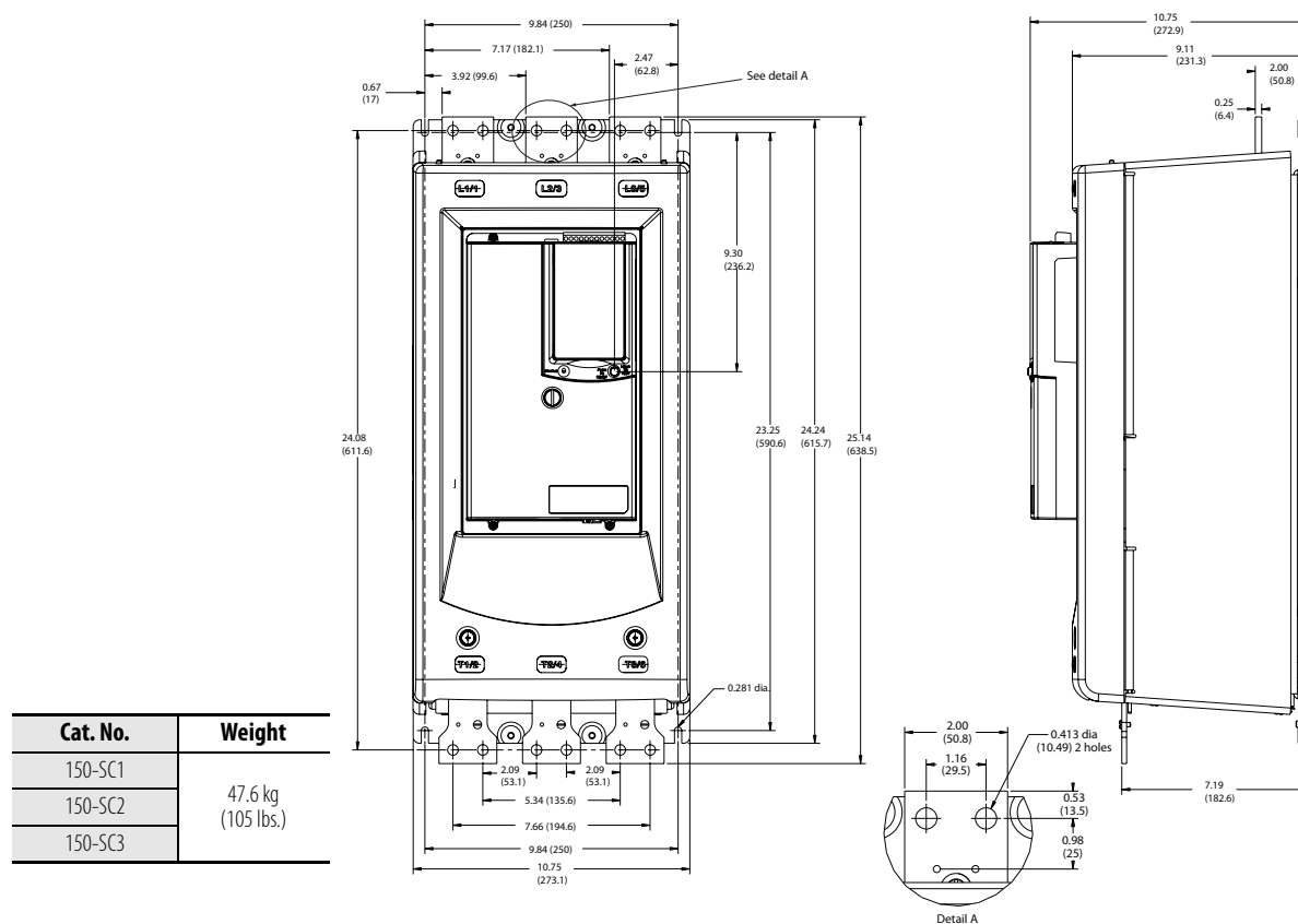
Figure 31 - Cat. Nos. 150-SC1...SC3 Solid-state Controller
