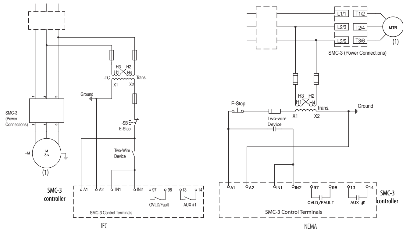
Figure 1 - Two-wire Configuration
