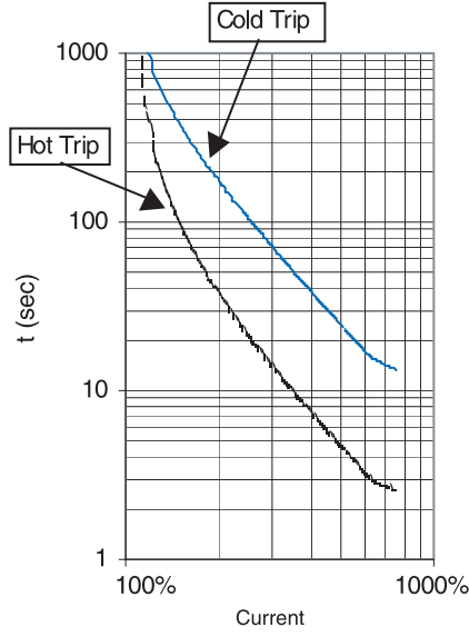
Trip Class 20
