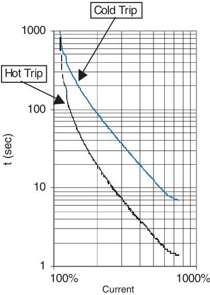
Trip Class 10
