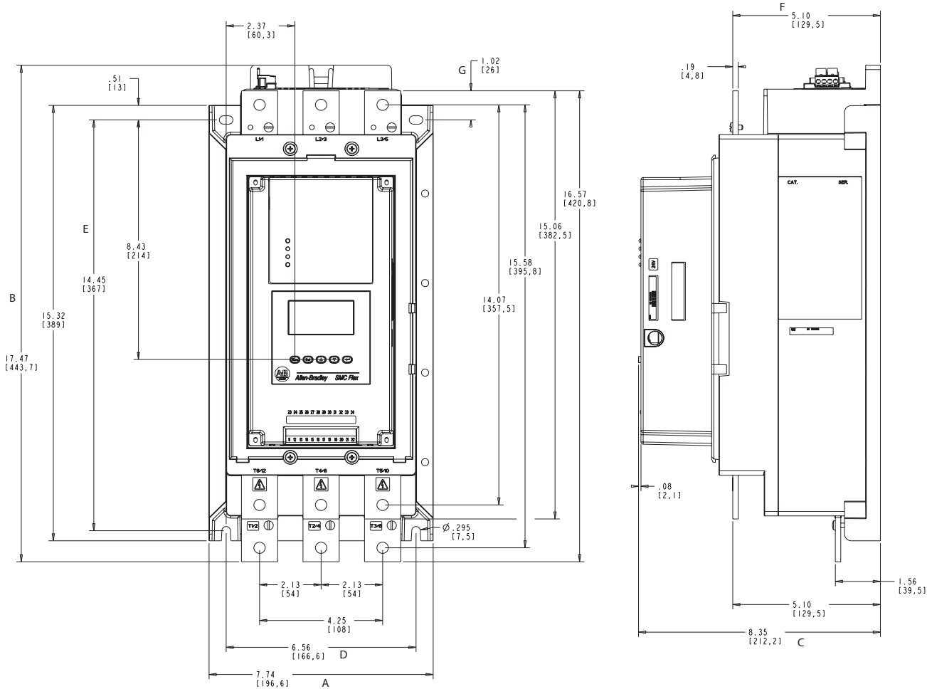
Figure 14 - 108...135 A Controllers
