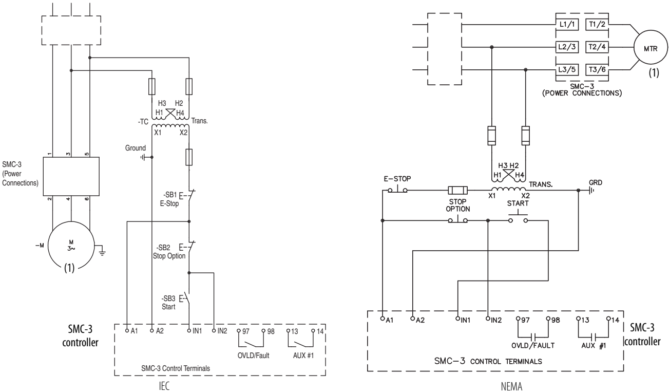
Figure 2 - Three-wire Configuration
