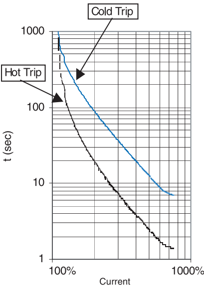
Trip Class 10
