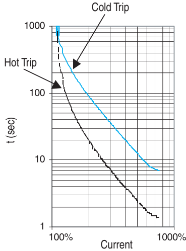
Trip Class 10
