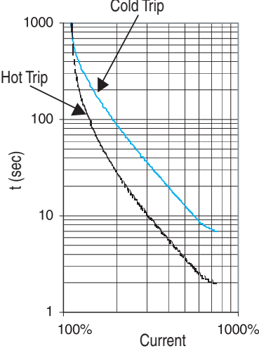
Trip Class 15
