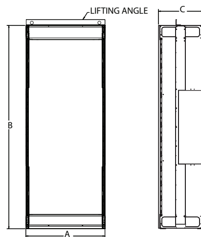
Figure 4 — Floor-Mount
