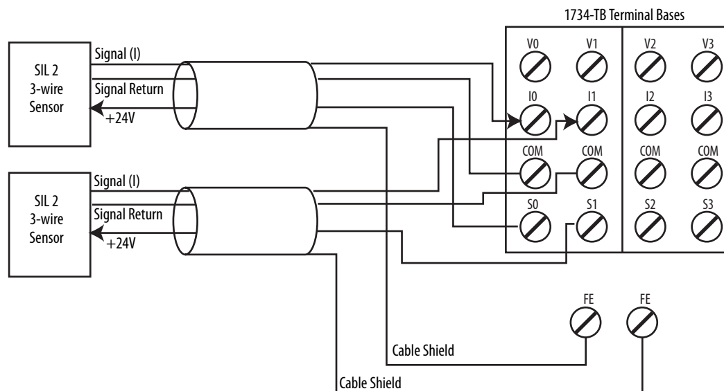
Figure 42 - 3-wire Current Sensor (SIL 3)
