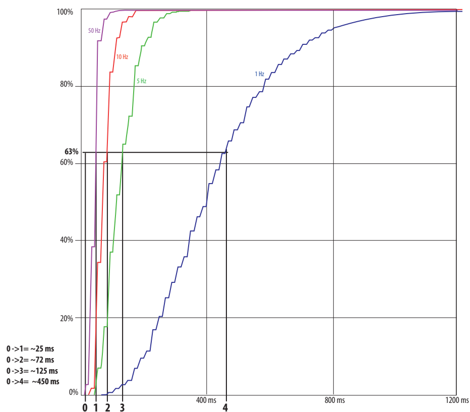
Figure 53 - Step Response
