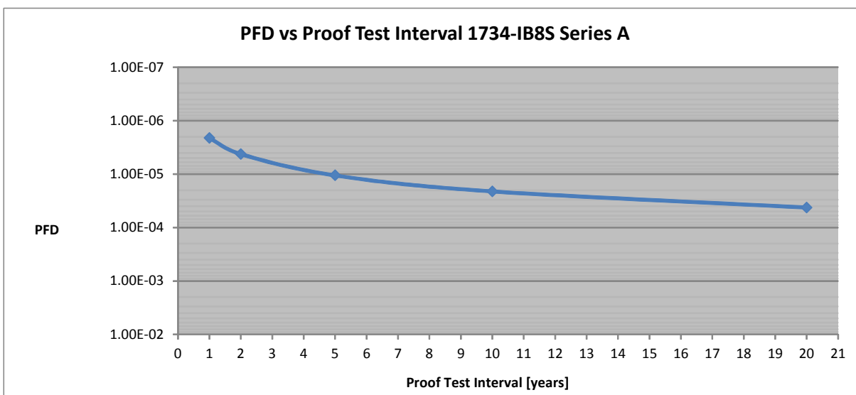
Figure 64 - PFD vs. Proof Test Interval 1734-IB8S Series A
