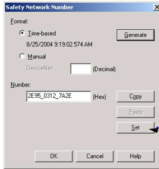
Figure 49 - Setting the SNN with a GuardLogix Controller
