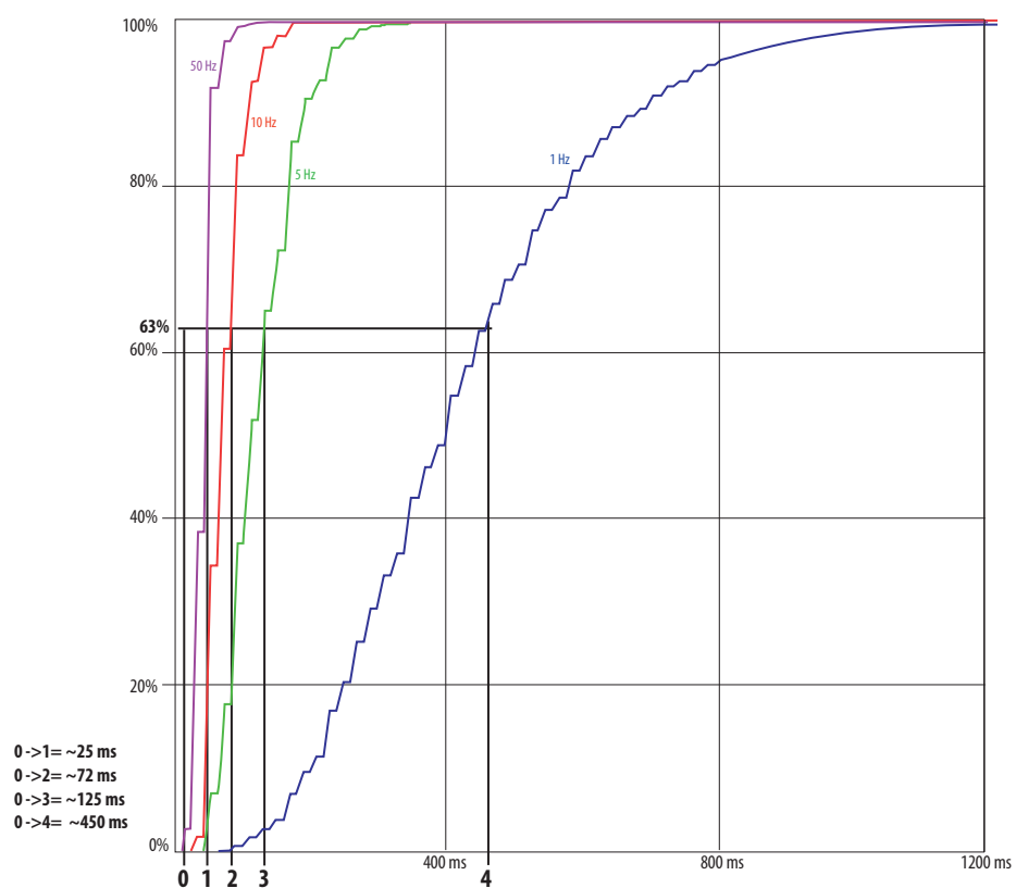
Figure 53 - Step Response
