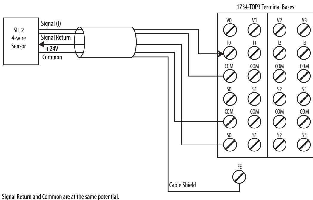
Figure 39 - 4-wire Current Sensor (SIL 2)
