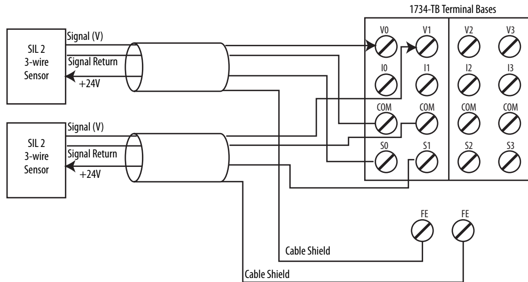
Figure 41 - 3-wire Voltage or Tachometer Sensor (SIL 3)
