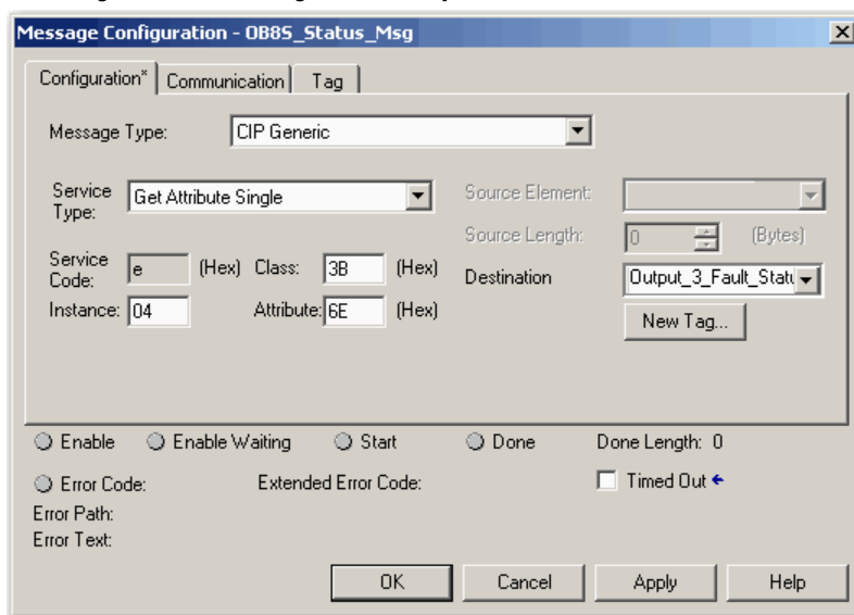
Figure 52 - Message Instruction Configuration Example
