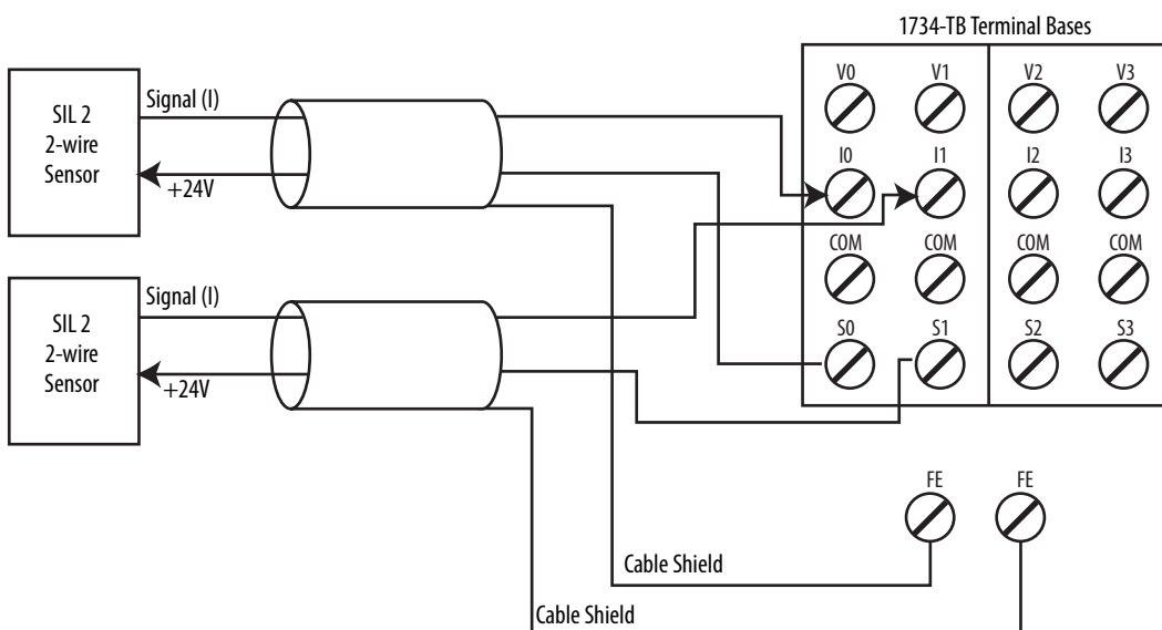
Figure 40 - 2-wire Current (4...20 mA) Sensor (SIL 3)
