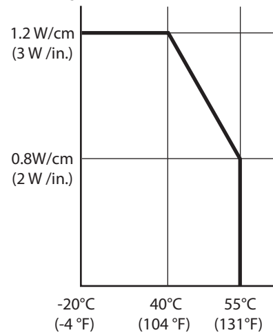
Figure 63 - System Temperature Derating When a 1734-IE4S Module Is Used
