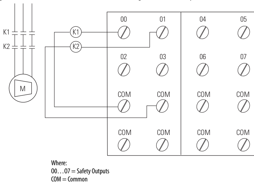
Figure 32 - 1734-OB8S POINT Guard I/O Module Wiring (redundant safety contacts)
