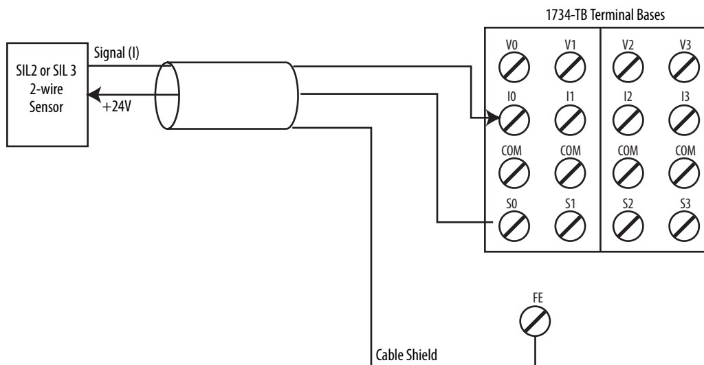
Figure 35 - 2-wire Current (4...20 mA) Sensor (SIL2 or SIL 3)
