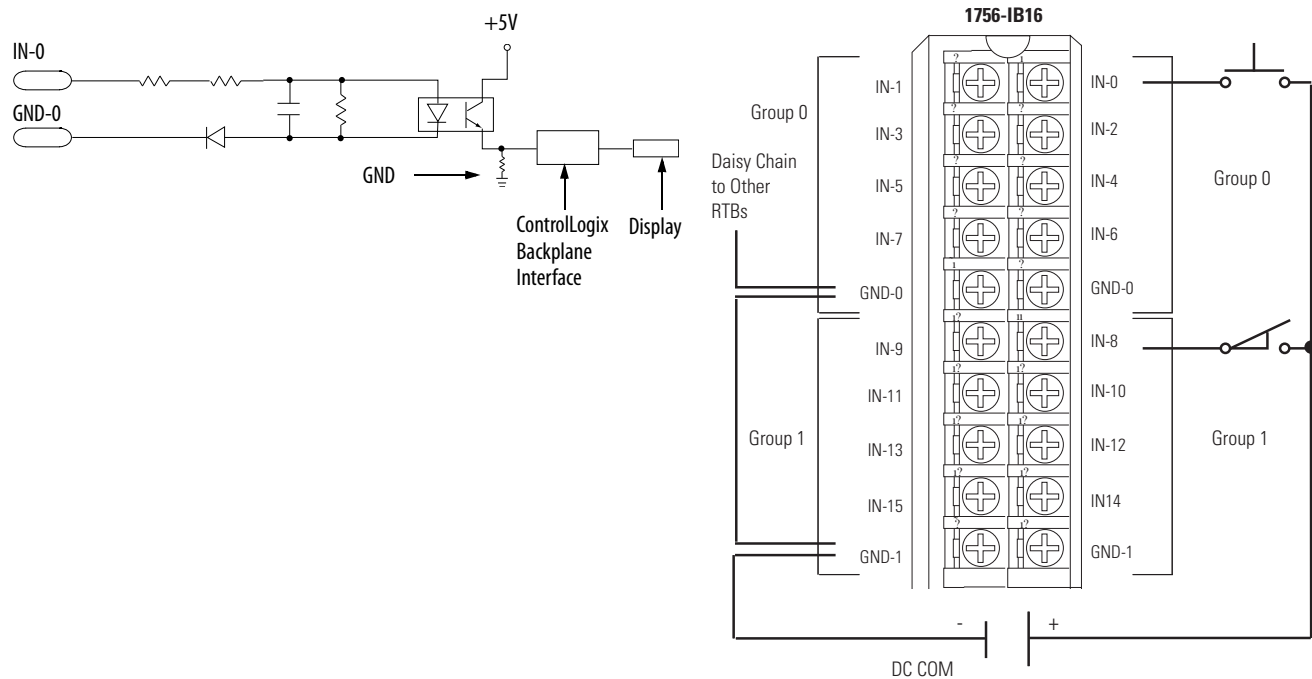
Simplified Schematic
