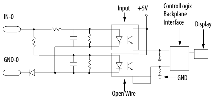
Simplified Schematic
