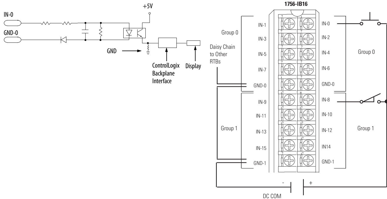
Simplified Schematic
