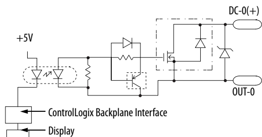
Simplified Schematic
