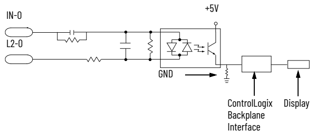
Simplified Schematic
