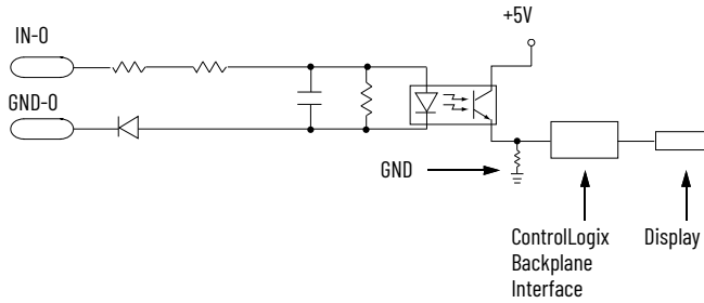
Simplified Schematic
