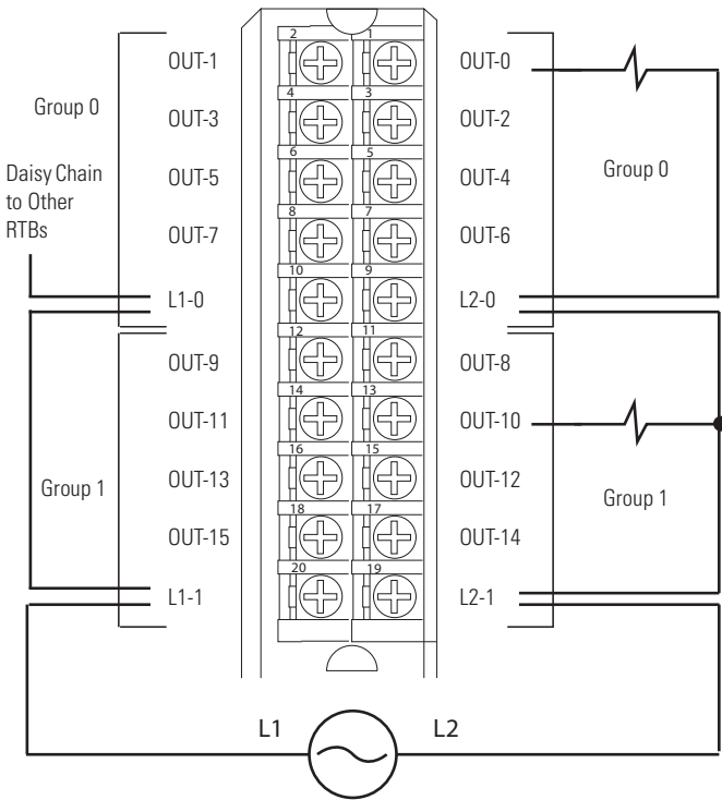
1756-0A16
