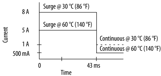
Surge Current Chart
