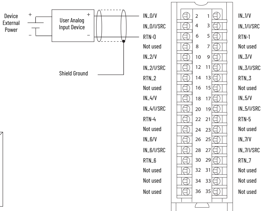
1756-IF8I, 1756-IF8IK Module Wiring Diagram - Voltage Mode
