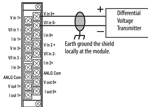
1769-IF4X0F2 Differential Inputs
