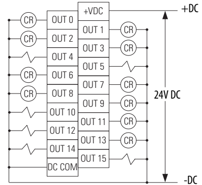
1769-OB16P
