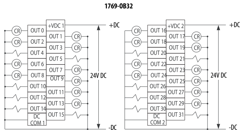
Simplified Output Circuit Diagram
