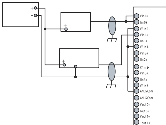
1769-IF4FX0F2F Single-ended Sensor/Transmitter Inputs
