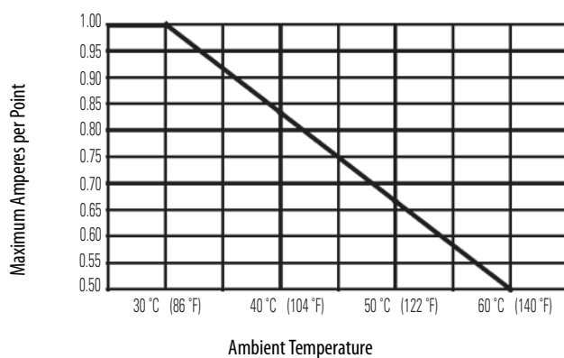
1769-BOOLEAN Maximum Amperes per Module Versus Temperature
