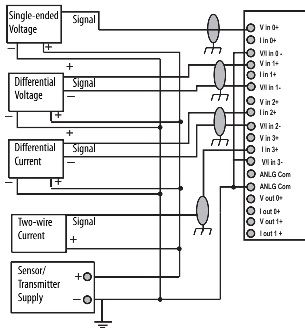
1769-IF4X0F2 Mixed Transmitter Inputs
