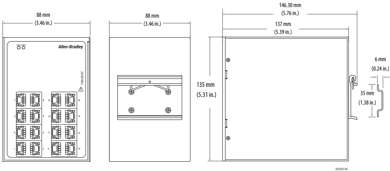
Figure 9 - 1783-US16T/A, 1783-US14T2S/A, 1783-US6TG2CG/A Switch Dimensions
