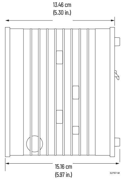
All Switches and Expansion Modules
