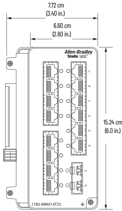
16-port Expansion Modules 1783-MMX16T, 1783-MMX16E, 1783-MMX14T2S
