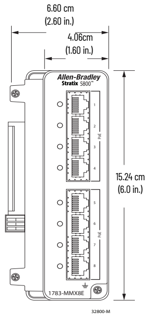
8-port Expansion Modules 1783-MMX8T, 1783-MMX8E, 1783-MMX8EA, 1783-MMX8S, 1783-MMX8SA, 1783-MMX6T2S
