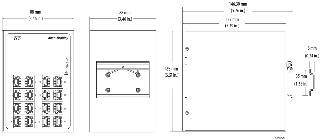
Figure 9 - 1783-US16T/A, 1783-US14T2S/A, 1783-US6T62CG/A Switch Dimensions
