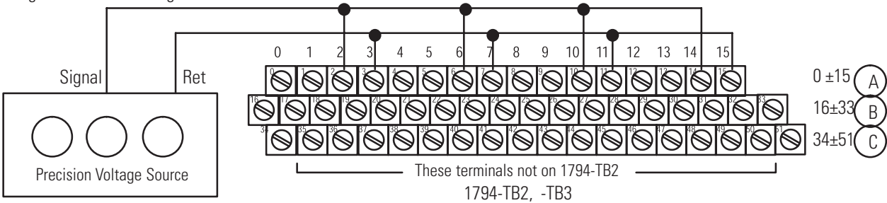
Figure 7.1 Calibration Set-Ups
