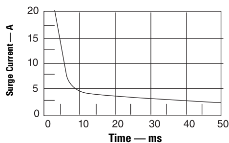
1794-OB8EP Output Minimum Surge
