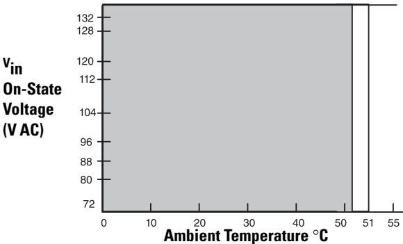
1794-OA16 Derating Curve
