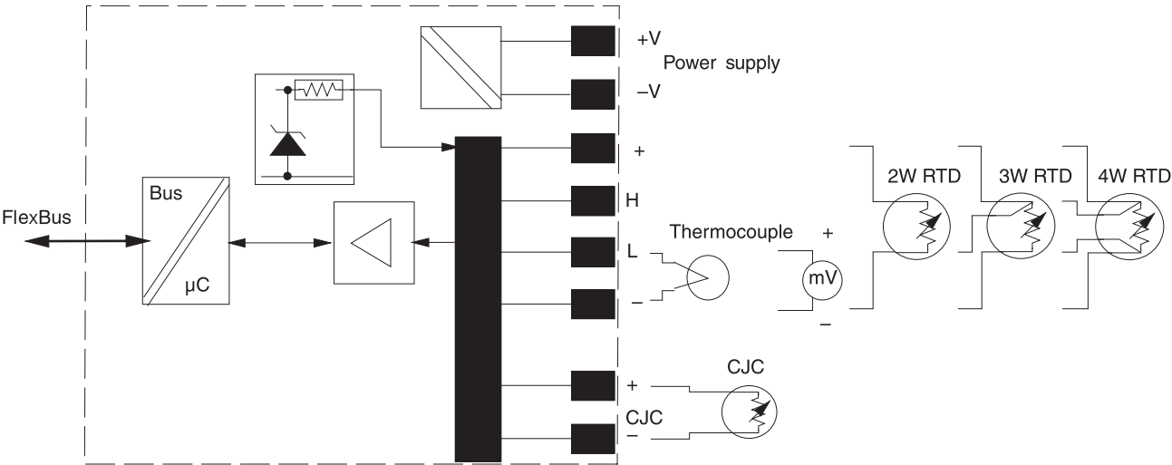
8 Point 16-bit Non-isolated RTD Thermocouple/mV Input Module
