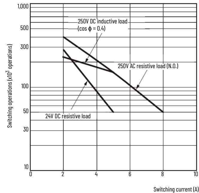
Micro810 Controller High Current Relay Chart
