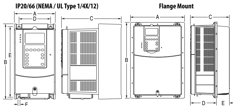
Frame Dimensions, mm (in.)
