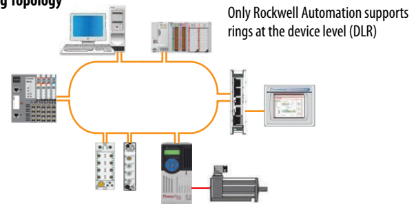
Ring Topology
