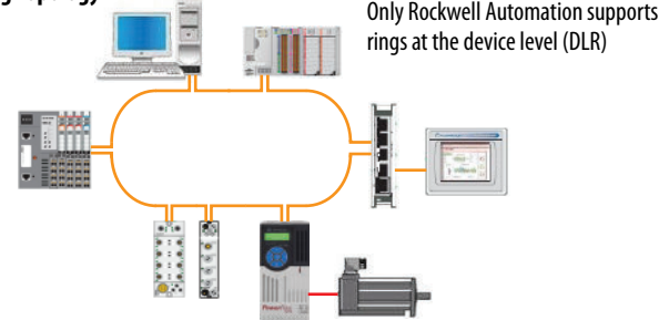
Ring Topology
