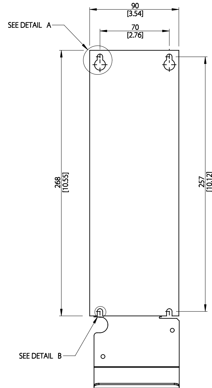
MOUNTING BASE
