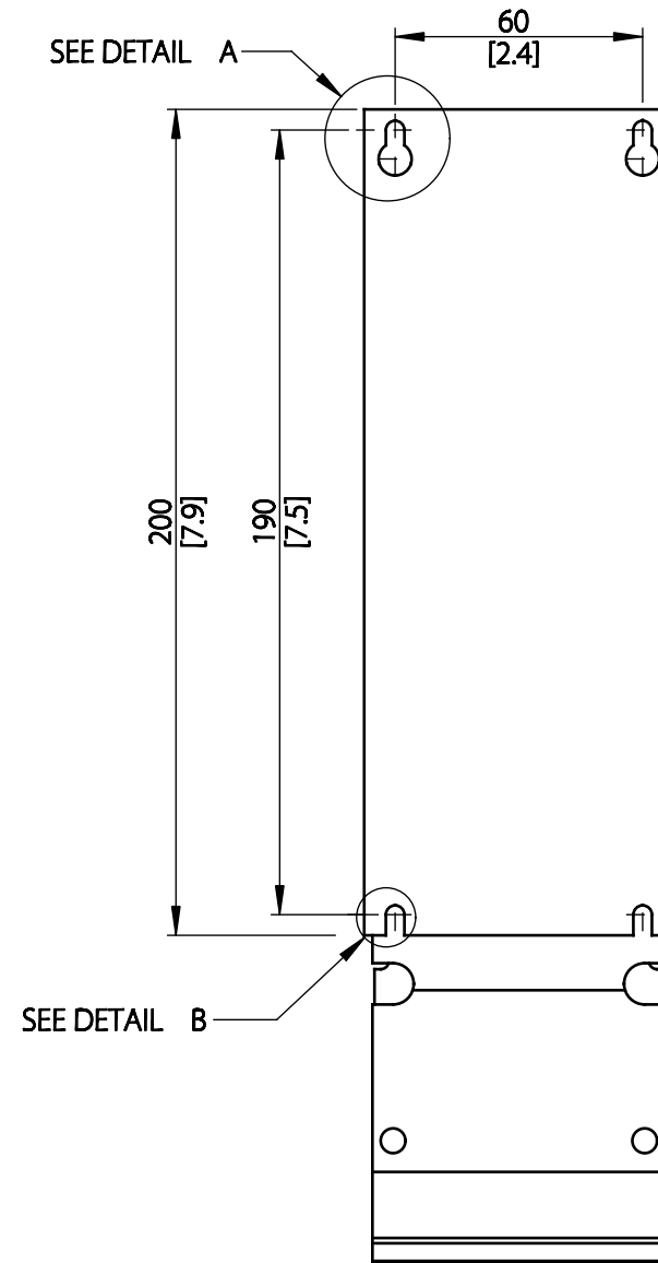
MOUNTING BASE
