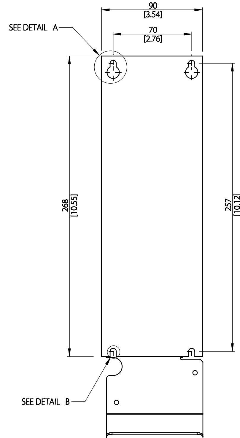
MOUNTING BASE
