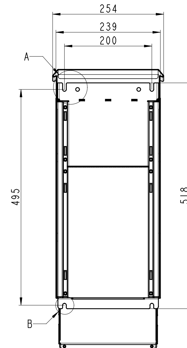
Mounting Base
