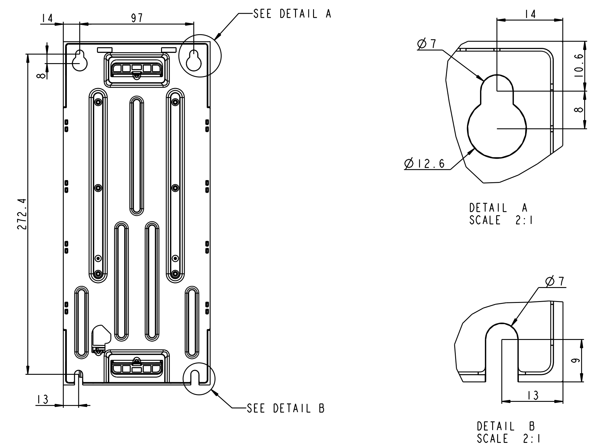
MOUNTING-BASE
