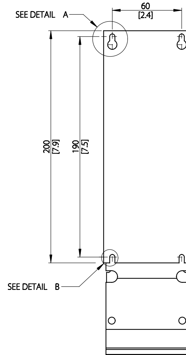
MOUNTING BASE
