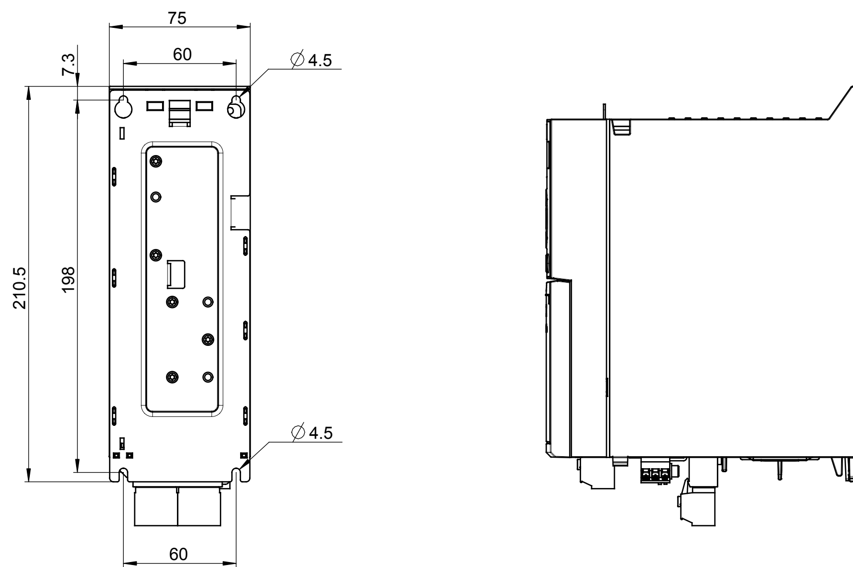
Mounting-Base
