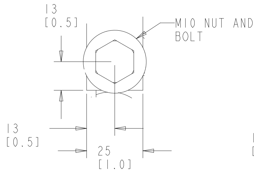
MAINS TERMINAL
