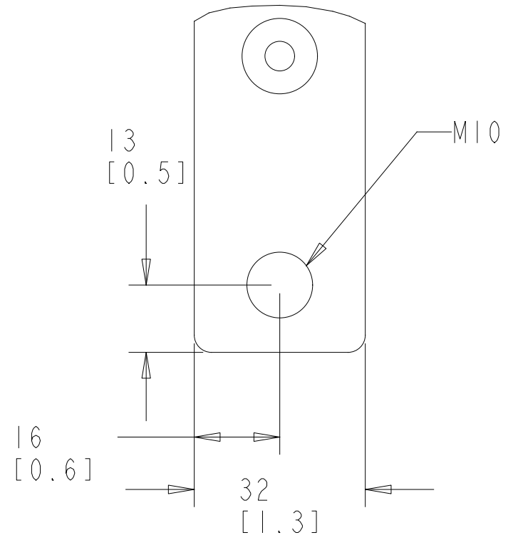
MOTOR TERMINAL
