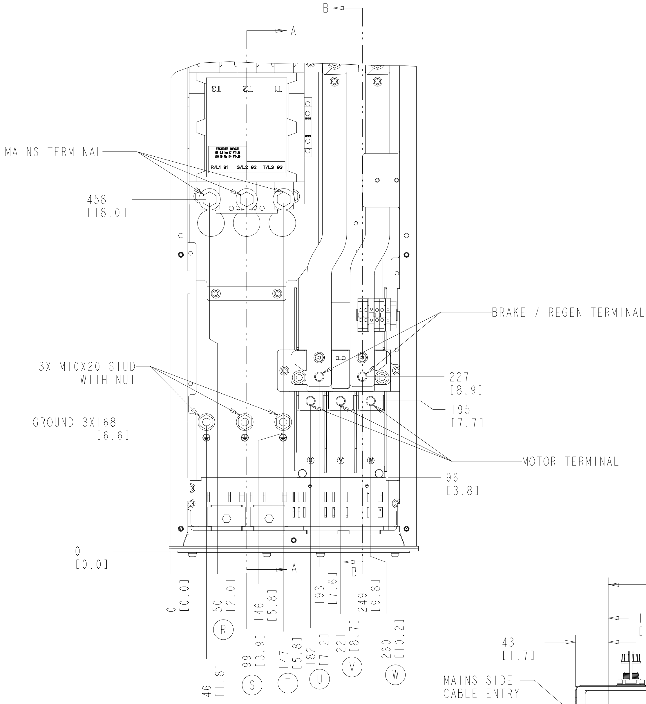
MOTOR TERMINAL
