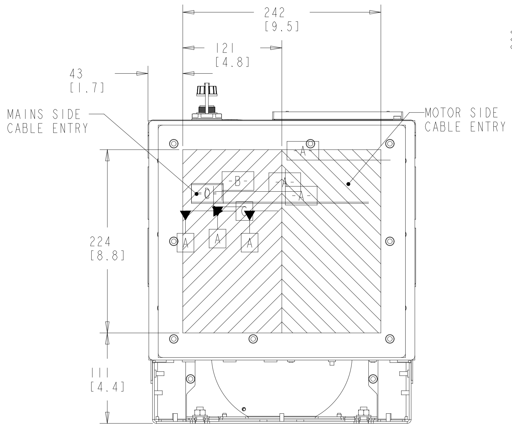
BOTTOM VIEW
