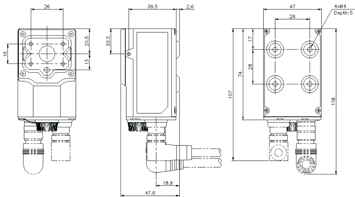
SR-1000+L-cable
