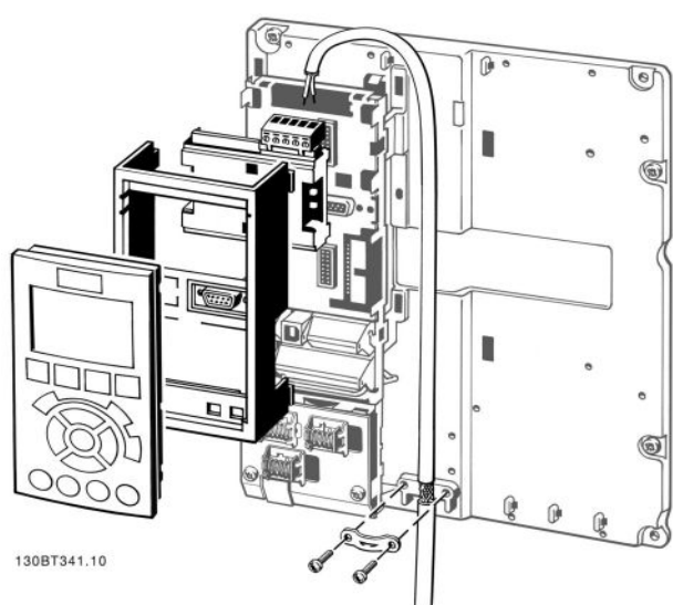
Illustration 3.3 Cable Holders
