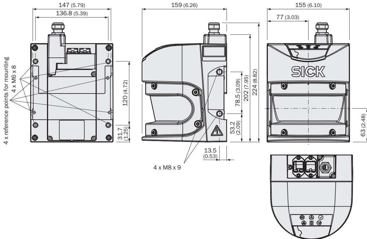
Dimensional drawing (Dimensions in mm (inch))
