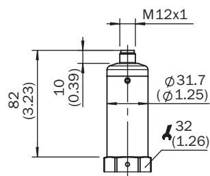
Dimensional drawing housing
