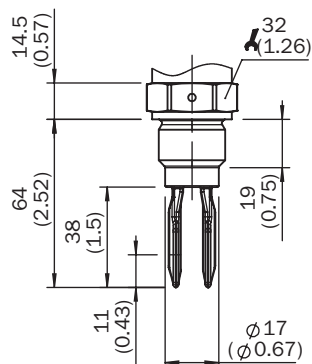
Dimensional drawing housing
