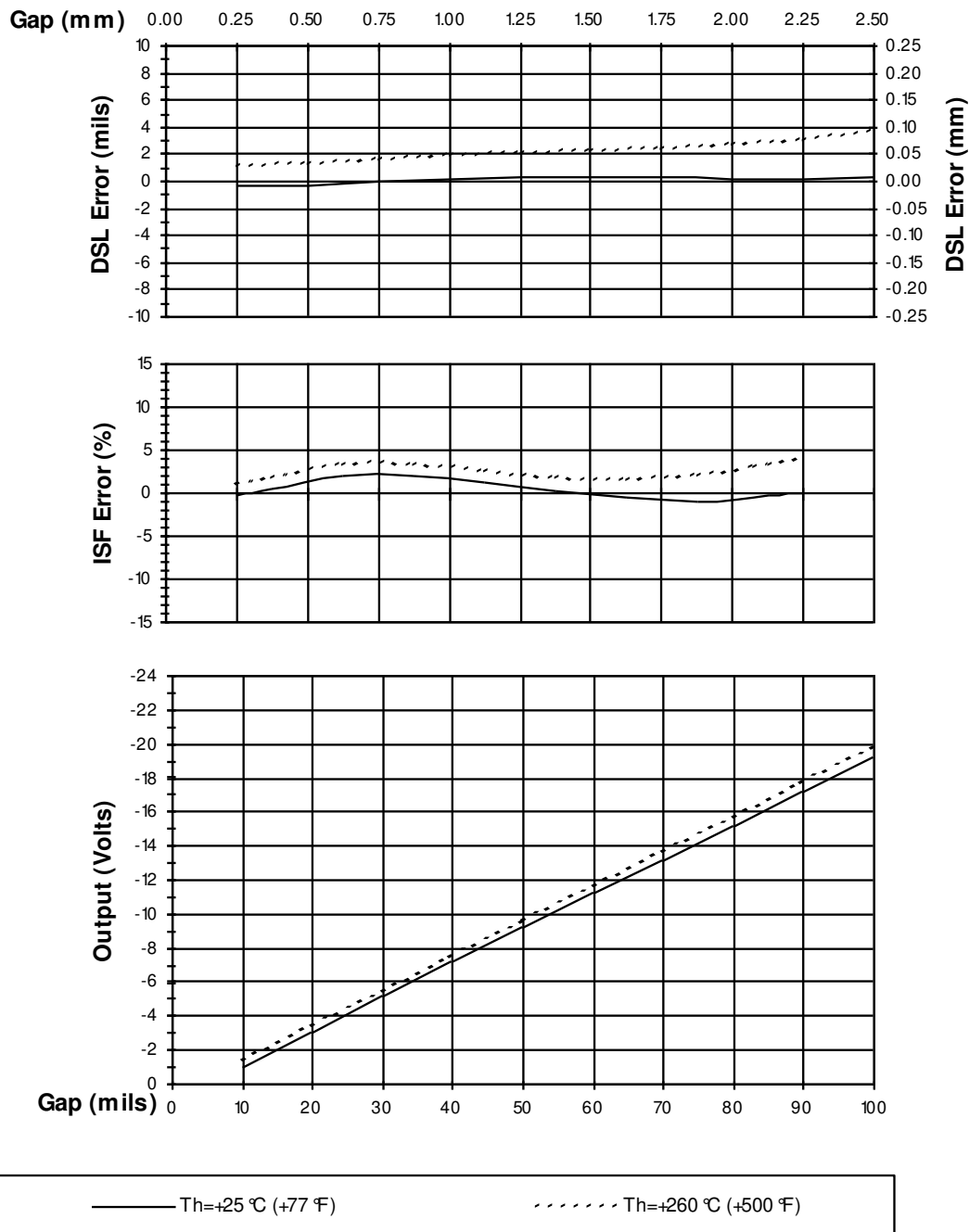
Figure 9: Typical 3300 XL Extended Temperature Range Probe and 8m Extended Temperature Range Extension Cable at T_h (Proximator Sensor and Probe Tip with 1-foot Cable are at +25\text{ }^{\circ}\text{C} )
