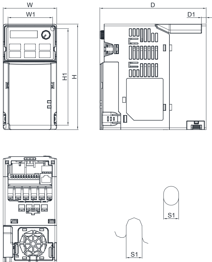
Mounting hole
