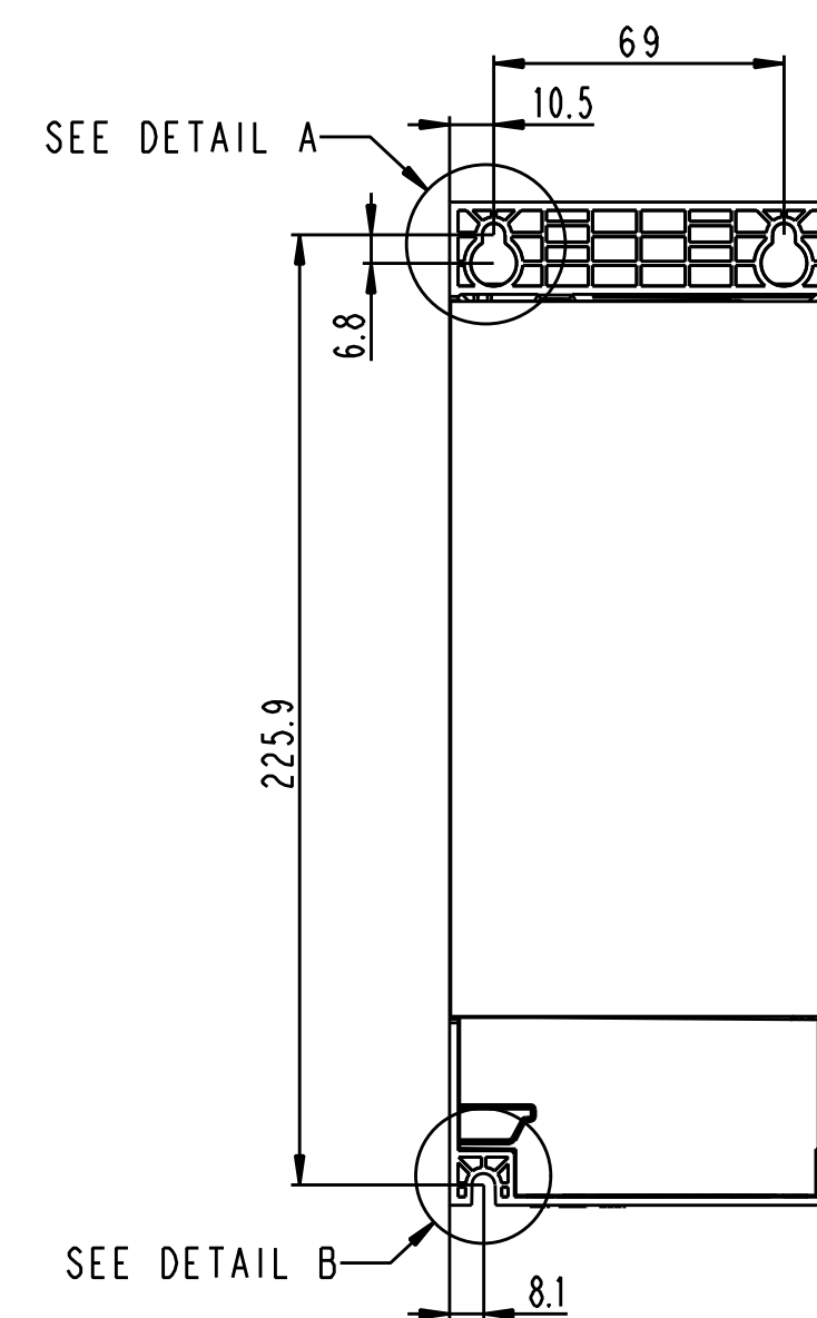
MOUNTING-BASE
