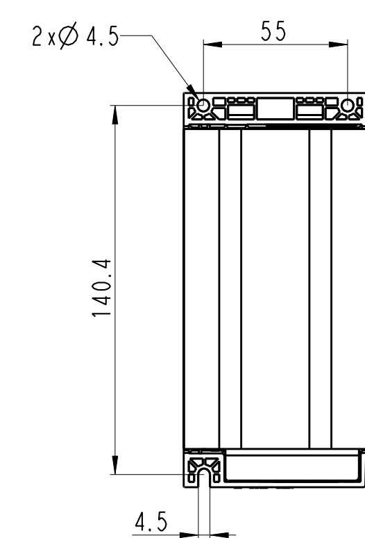
MOUNTING-BASE
