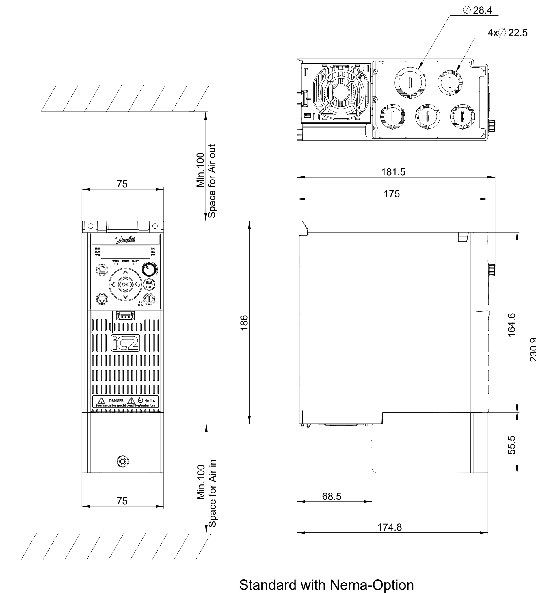
Standard with Nema-Option
