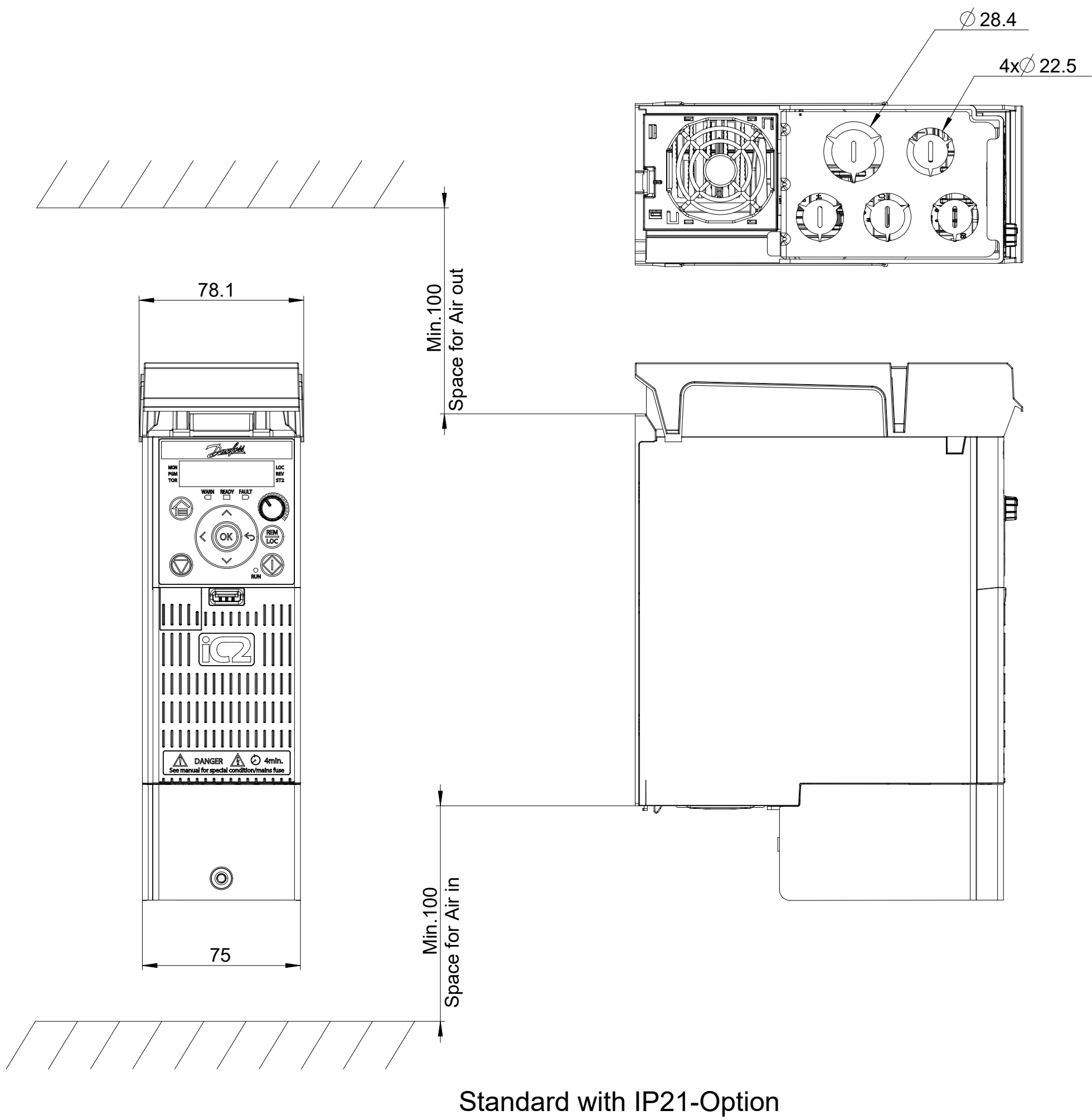
Standard with IP21-Option
