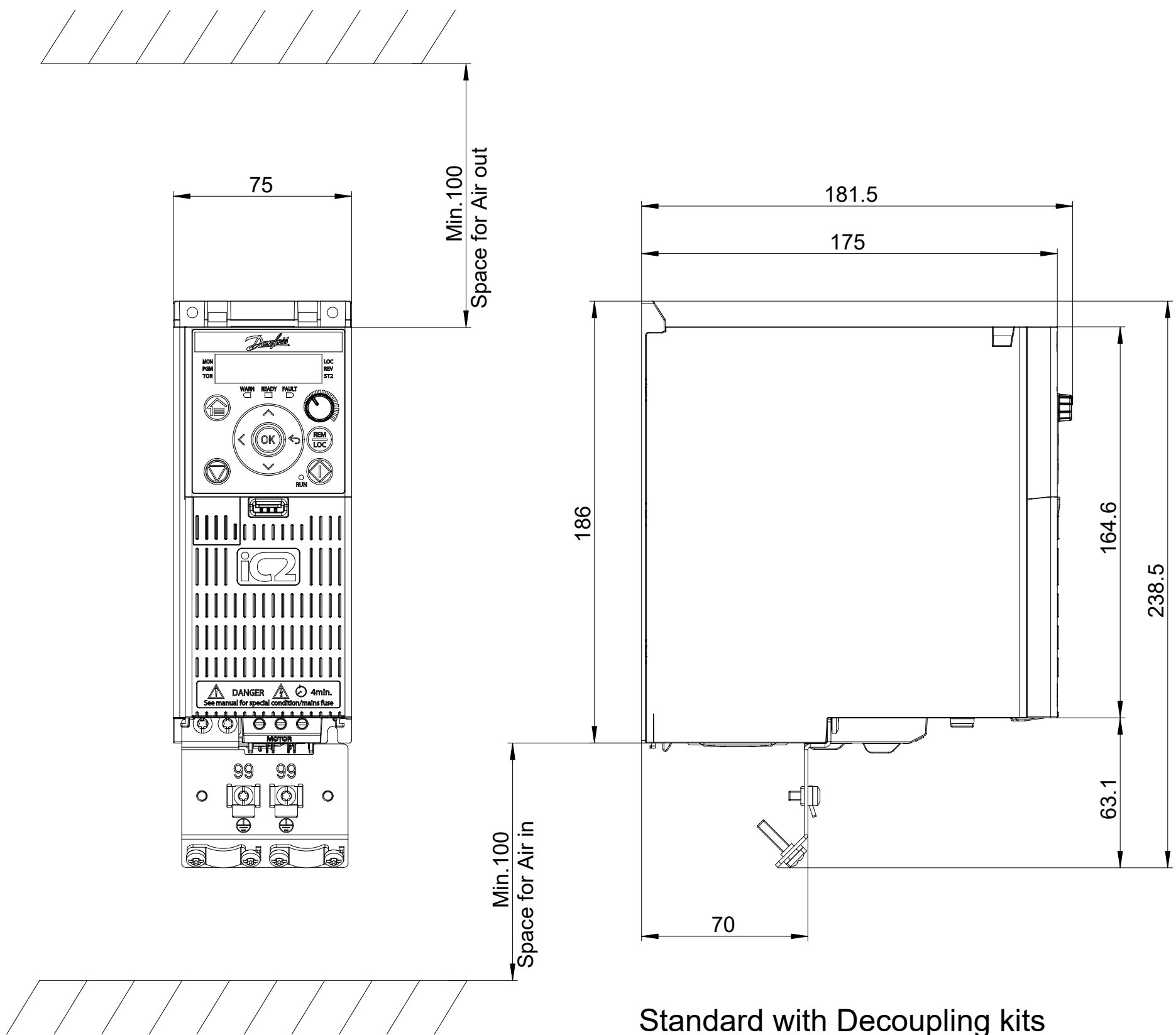
Standard with Decoupling kits
