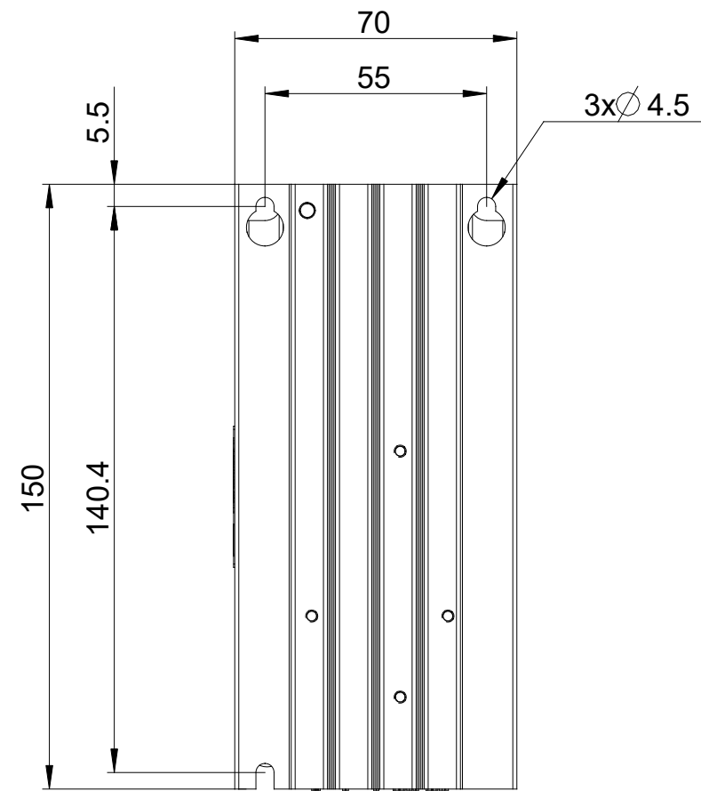
Mounting-Base
