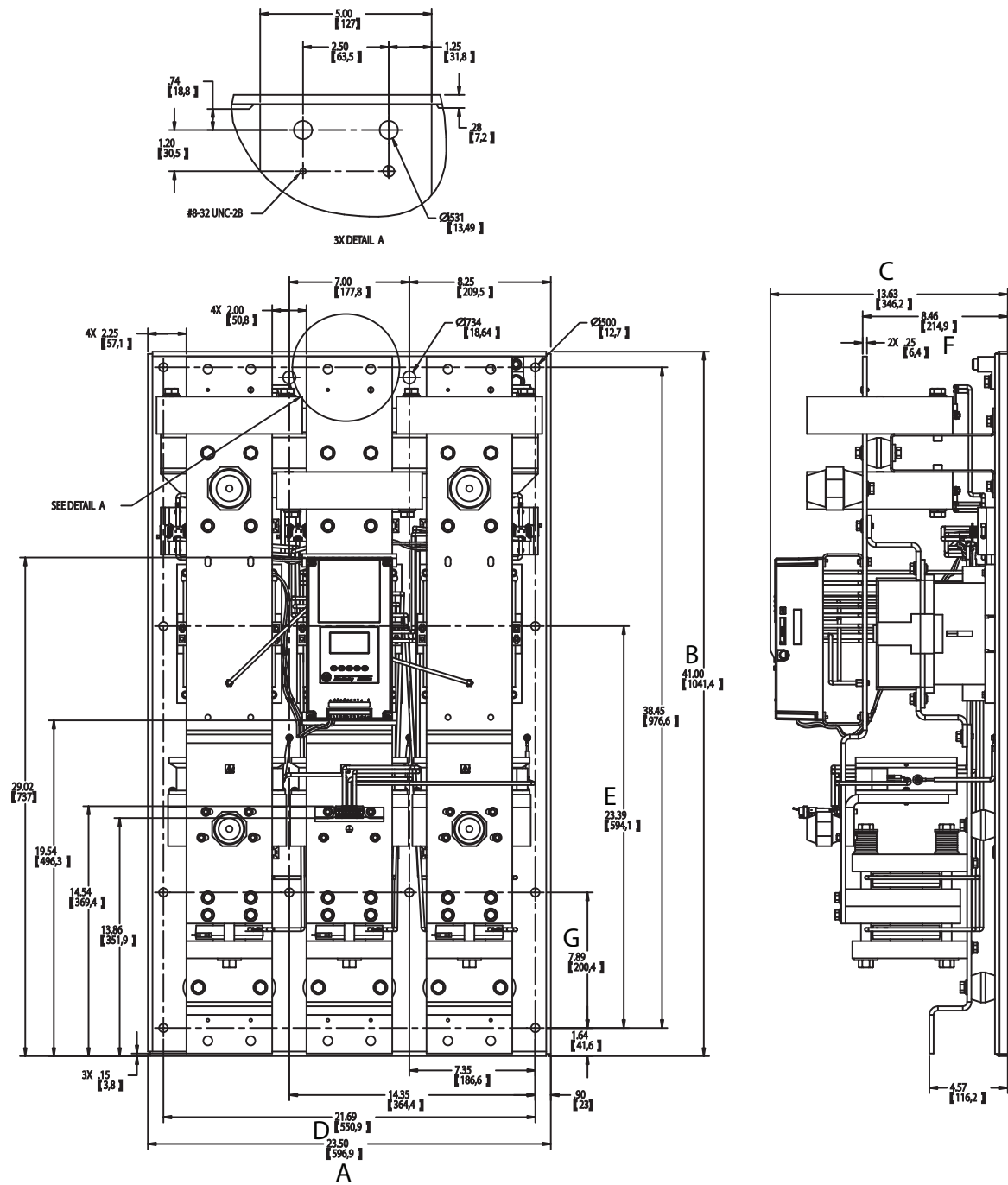
Figure 18 - 970...1250 A Controllers
