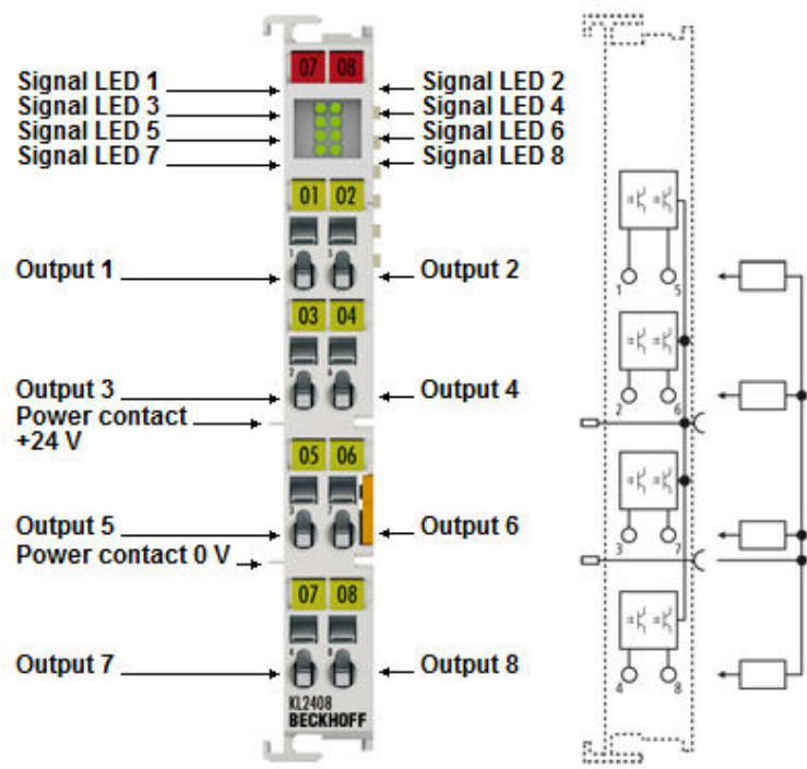
Fig. 28: KL2408 – Contact assignment and LEDs
