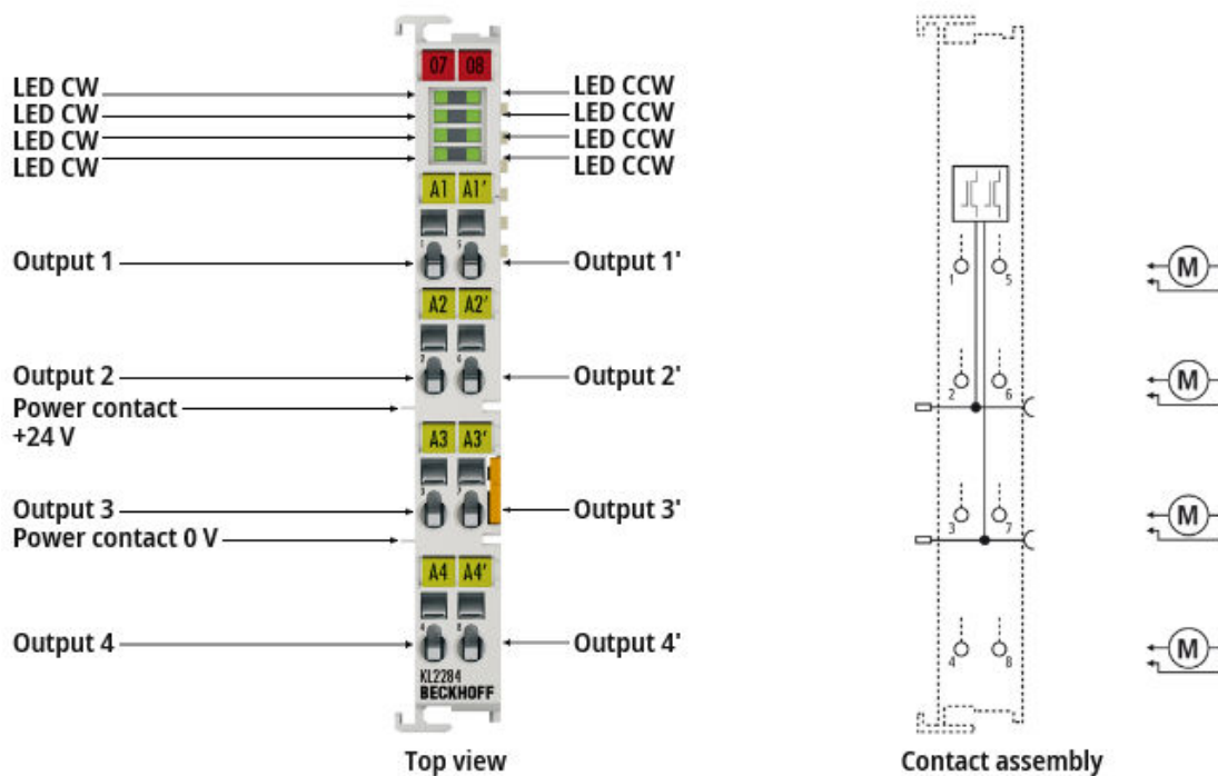
Fig. 21: KL2284 - Contact assignment and LEDs
