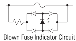
Blown Fuse Indicator Circuit
