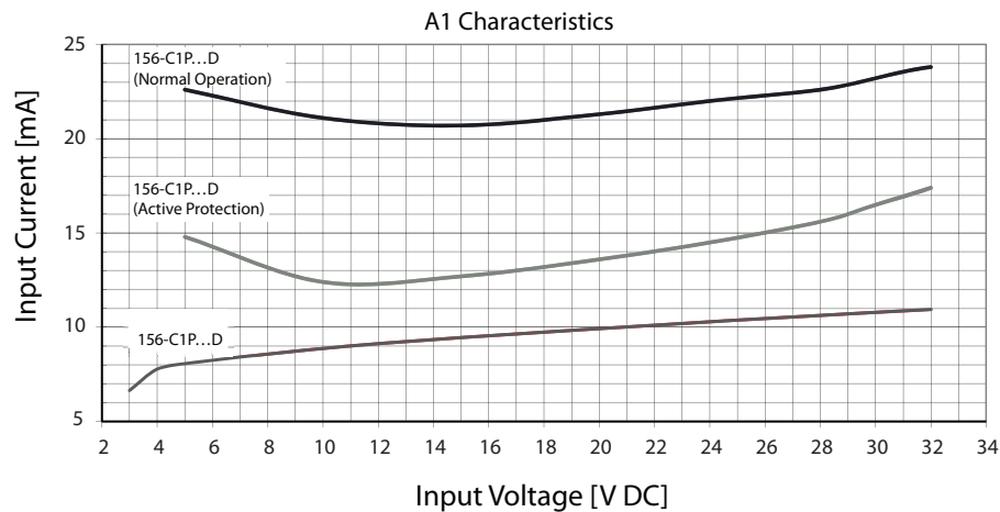
Figure 1 - 156-C1P...D Input Current vs. Input Voltage
