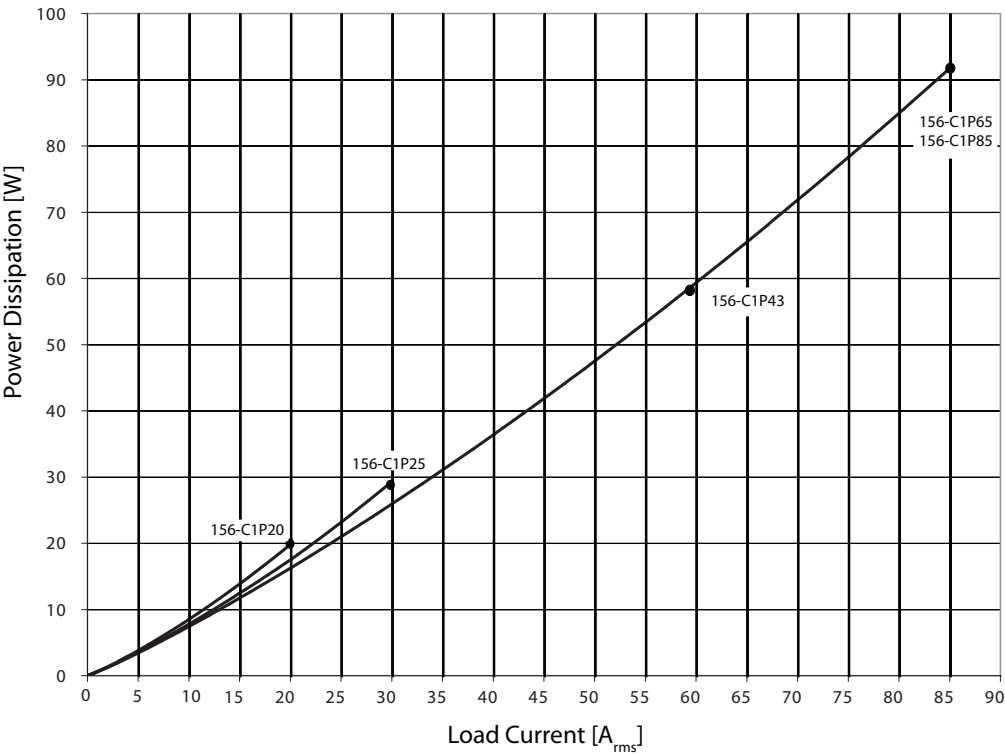
Figure 4 - Output Power Dissipation
