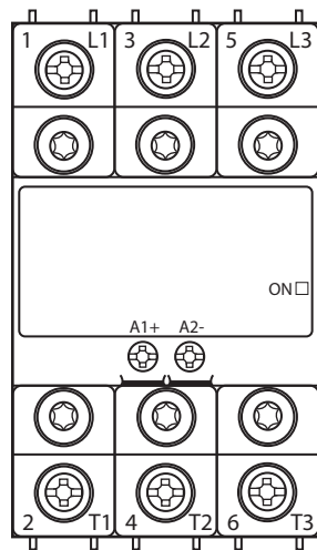
Figure 31 - Terminal Layout
