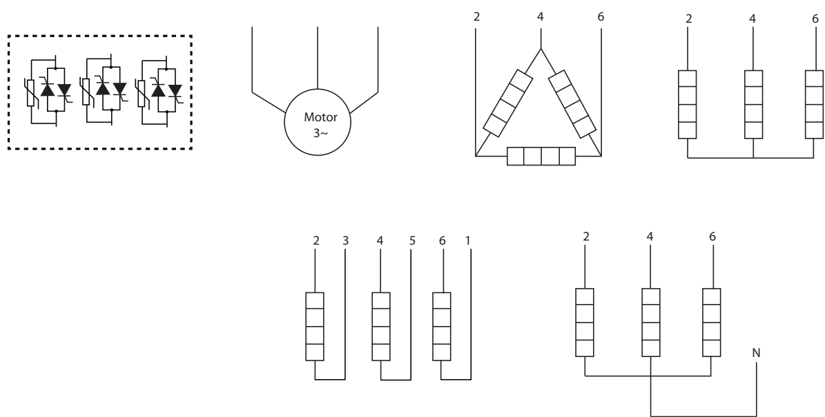
Figure 34 - Three-phase Connections
