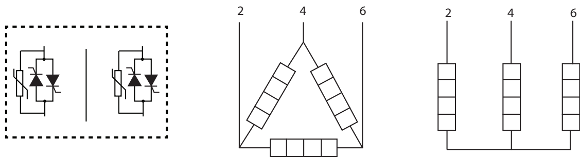
Figure 34 - Three-phase Connections
