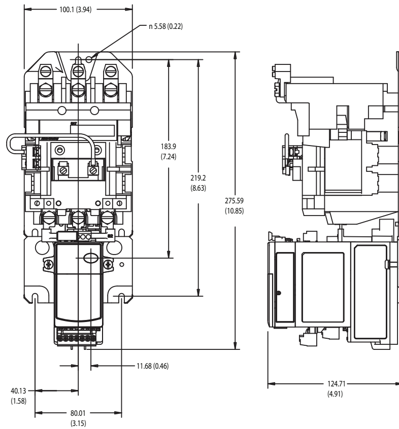
Figure 12 - E300 Overload Relay Mounted on Bulletin 500 NEMA Size 2 Contactor
