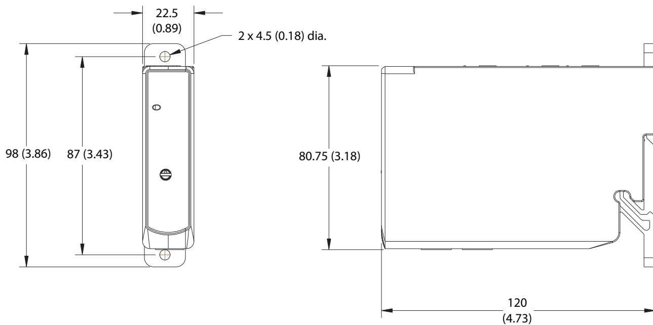
Figure 25 - E300 Analog Expansion Module 193-EXP-AIO-31
