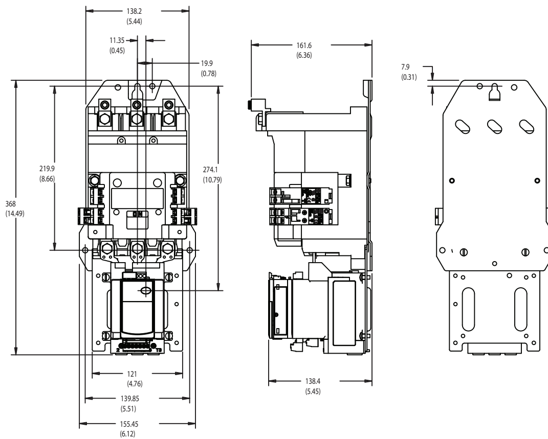
Figure 13 - E300 Overload Relay Mounted on Bulletin 500 NEMA Size 3 Contactor
