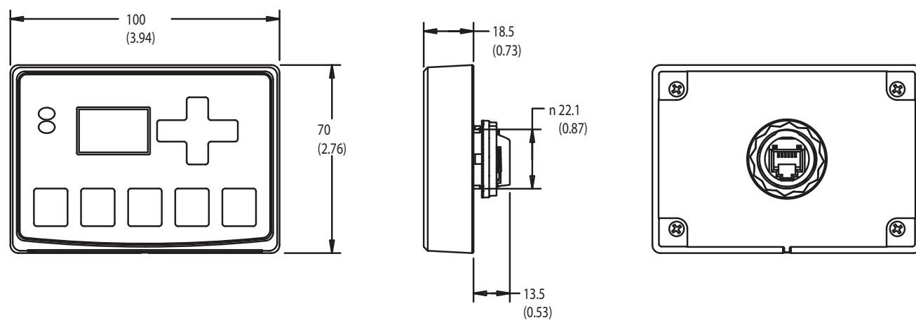
Figure 28 - E300 Starter Diagnostic Station 193-EOS-SDS
