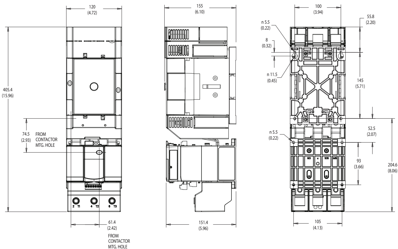
Figure 10 - E300 Sensing Module 193-ESM-___ - ___-D180 with 100-D115...-D180 Contactor and Terminal Covers
