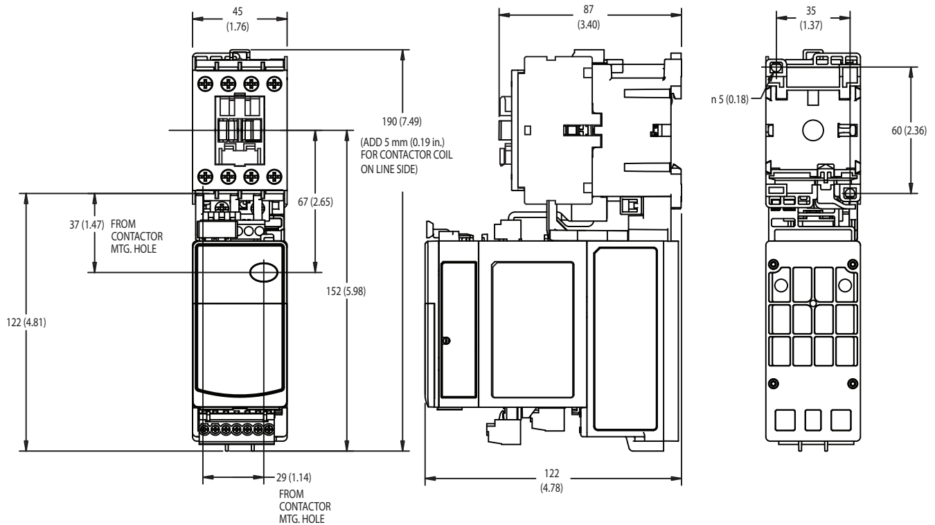
Figure 5 - E300 Overload Relay Mounted on Bulletin 100-C09...-C23 Contactor
