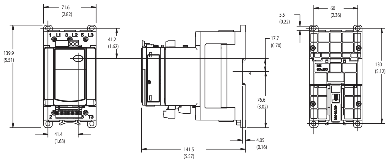
Figure 16 - E300 Overload Relay, 193-ESM-___ -100A-E3T, DIN Rail/Panel Mounted
