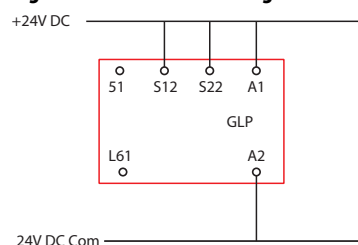
Figure 17 - No Guard Locking Connections
